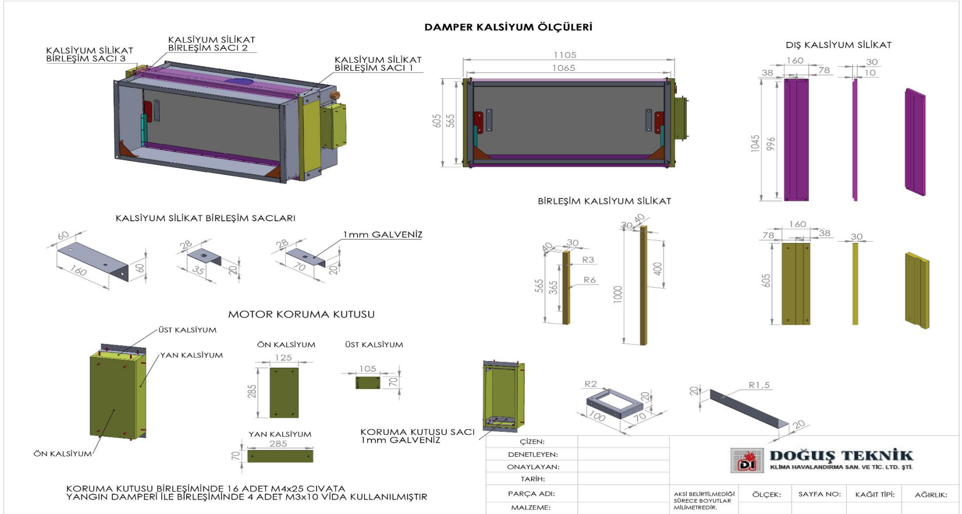
Figure 5: Overall dimensions and calcium silicate details of Damper A.
