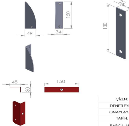
Figure 6: Overall dimensions and calcium silicate details of Damper A.
